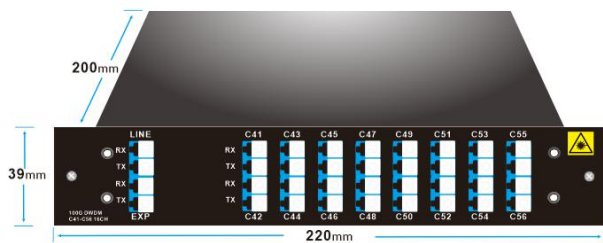
LGX BOX Plug in 2-Slot 1U Rack
