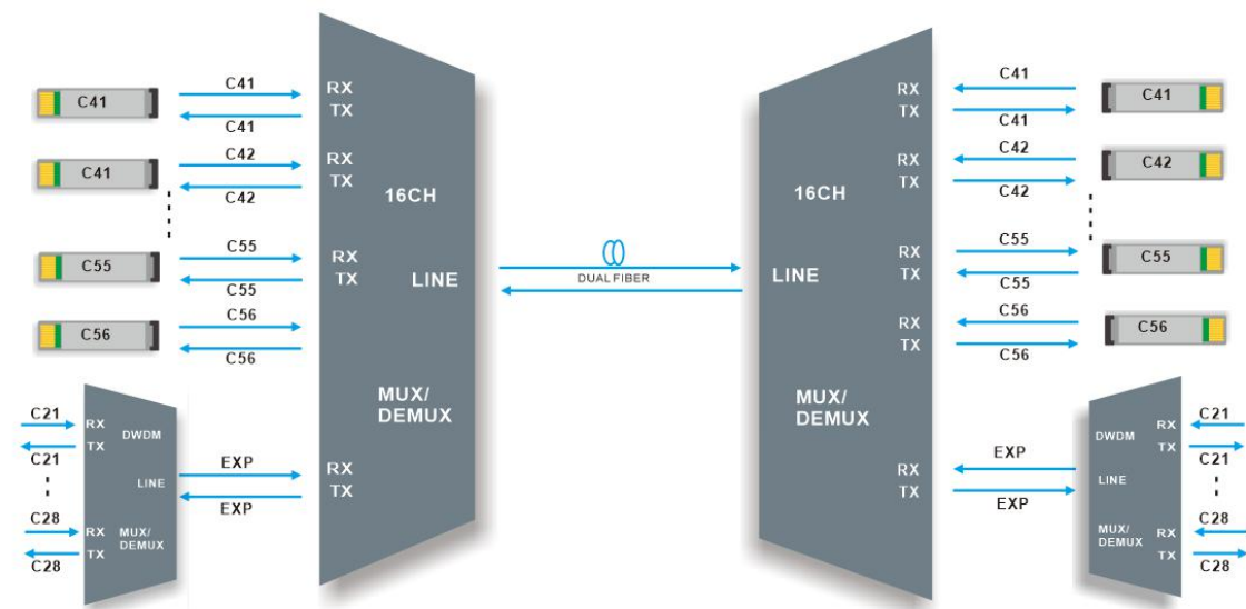
16CH DWDM MUX DEMUX Dual fiber transmission
