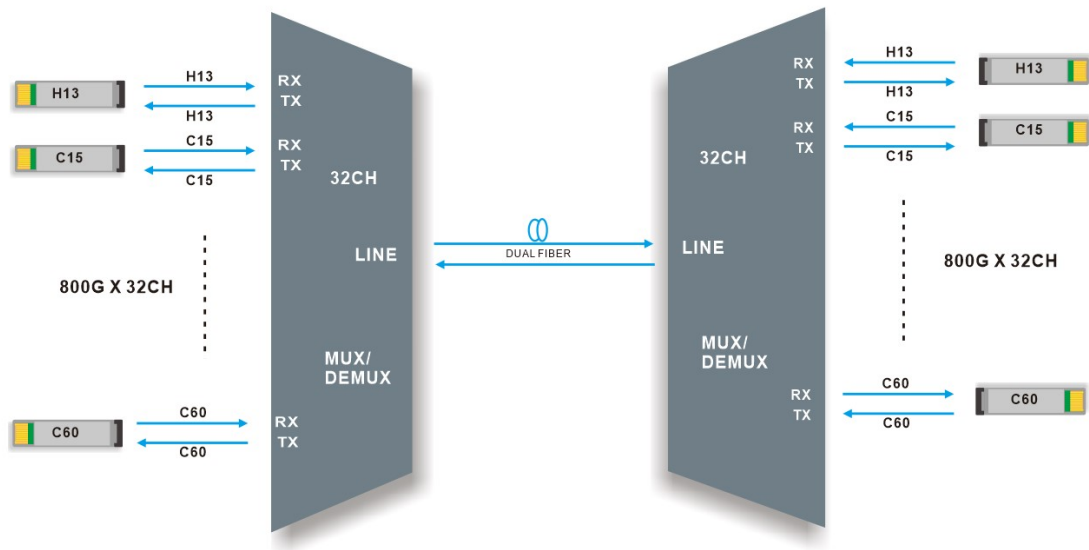
32CH DWDM MUX DEMUX Dual fiber transmission
